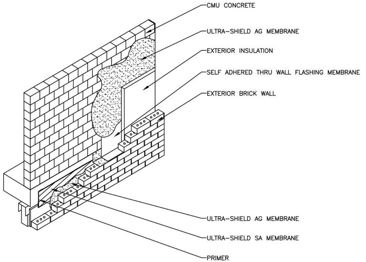
AIR BARRIER COLD CLIMATE W/CMU CONCRETE APPLICATION PROFILE ARCH. REF.:
